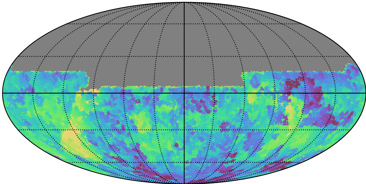
mw_roll_bulge_v3.3_10yrs All sky u band: Min fiveSigmaDepth
