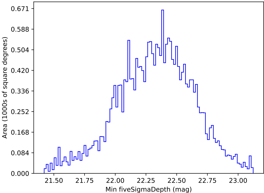
mw_roll_bulge_v3.3_10yrs All sky u band: Min fiveSigmaDepth
