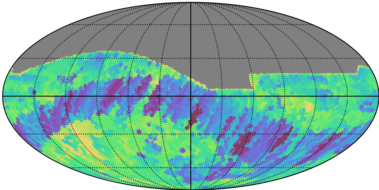
mw_roll_bulge_v3.3_10yrs All sky r band: Min fiveSigmaDepth
