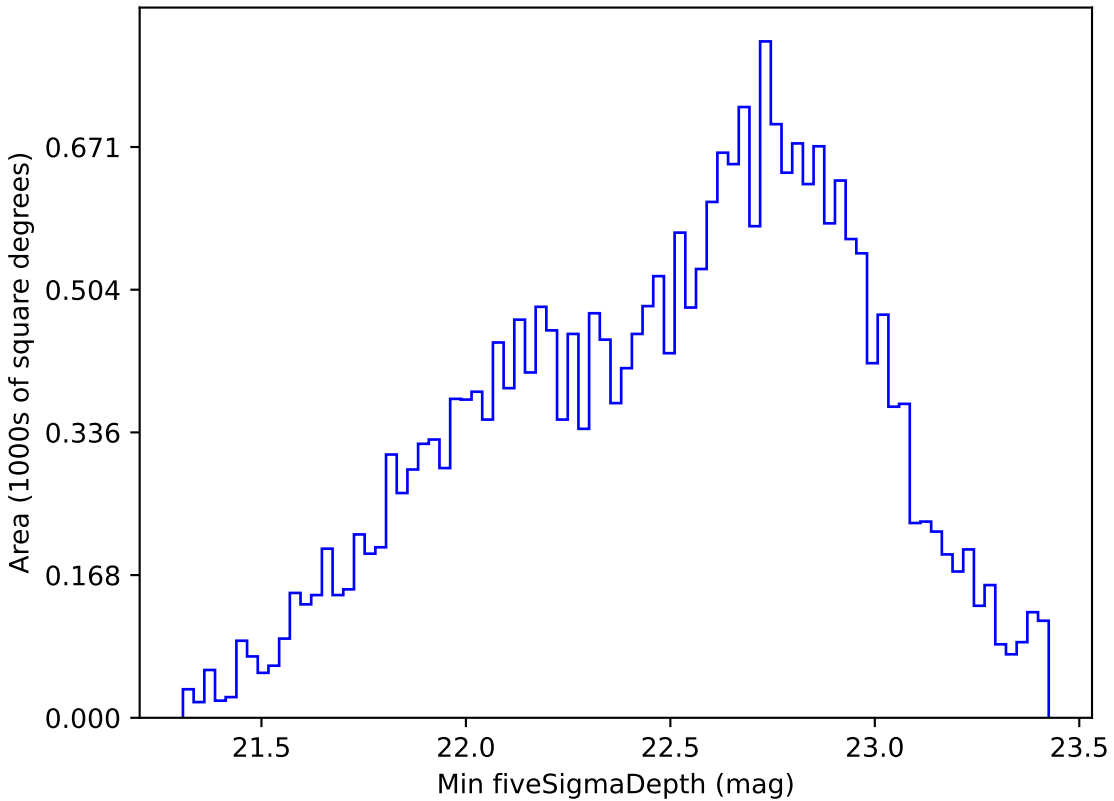
mw_roll_bulge_v3.3_10yrs All sky r band: Min fiveSigmaDepth
