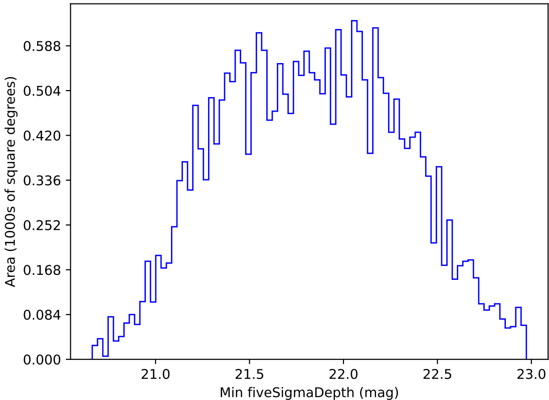
mw_roll_bulge_v3.3_10yrs All sky i band: Min fiveSigmaDepth
