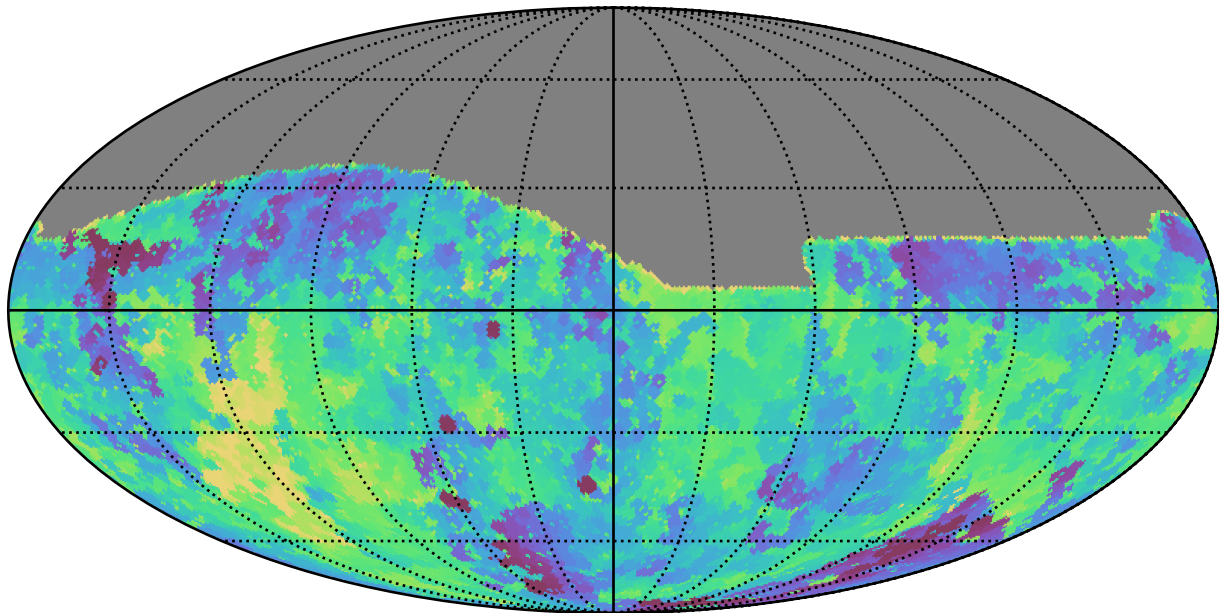
mw_roll_bulge_v3.3_10yrs All sky g band: Min fiveSigmaDepth
