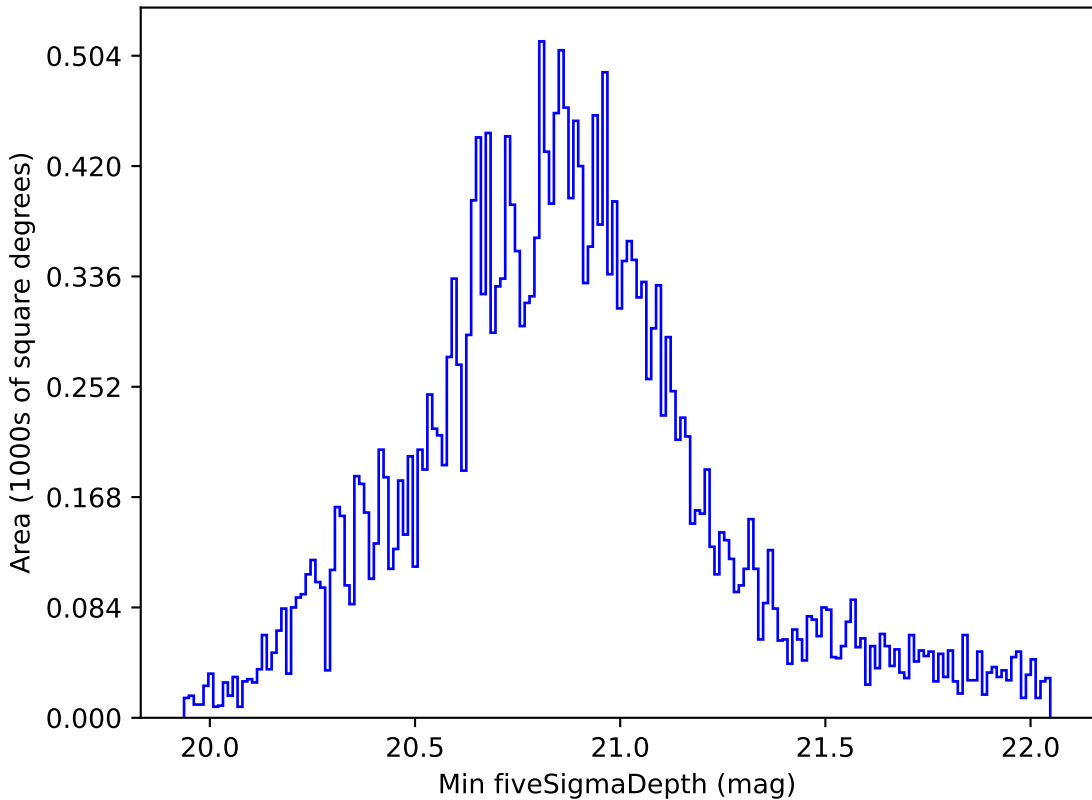
mw_roll_bulge_v3.3_10yrs All sky all bands: Min fiveSigmaDepth
