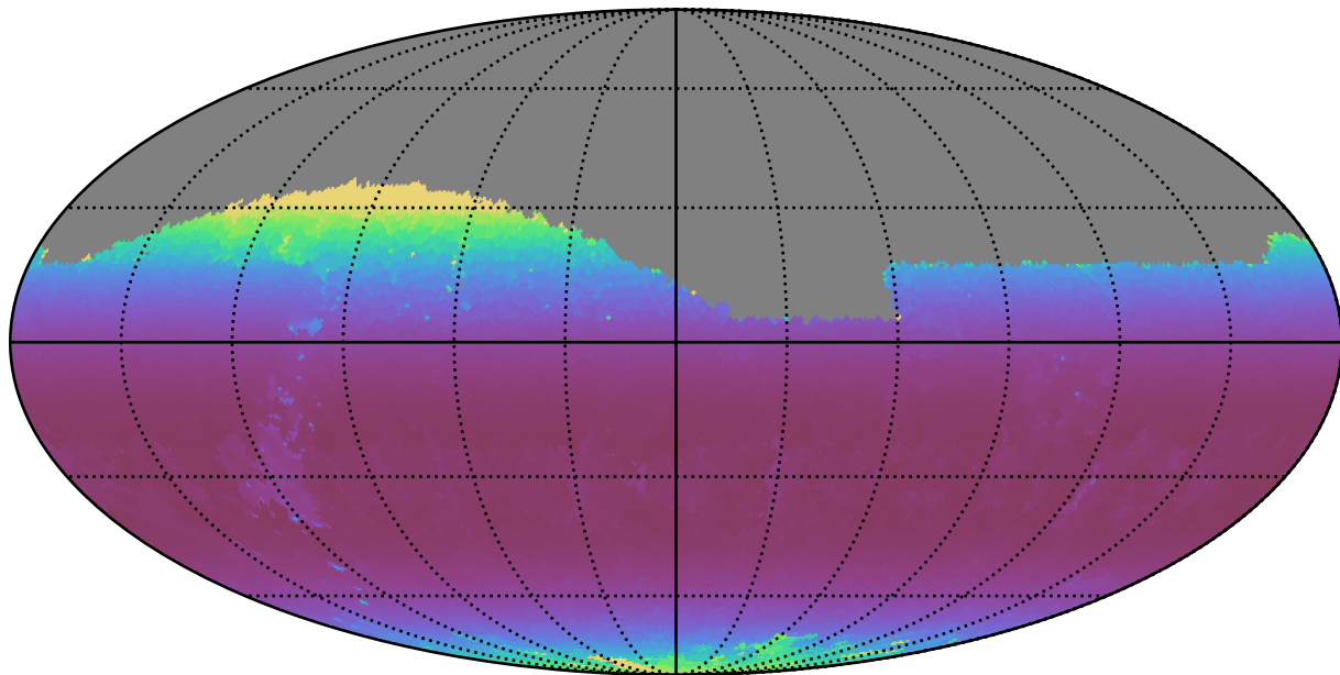
mw_roll_bulge_v3.3_10yrs Yr 1 z band: Min airmass
