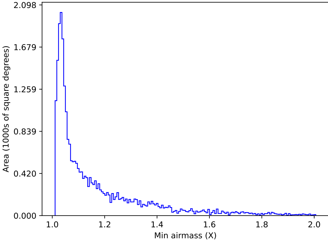
mw_roll_bulge_v3.3_10yrs Yr 1 z band: Min airmass
