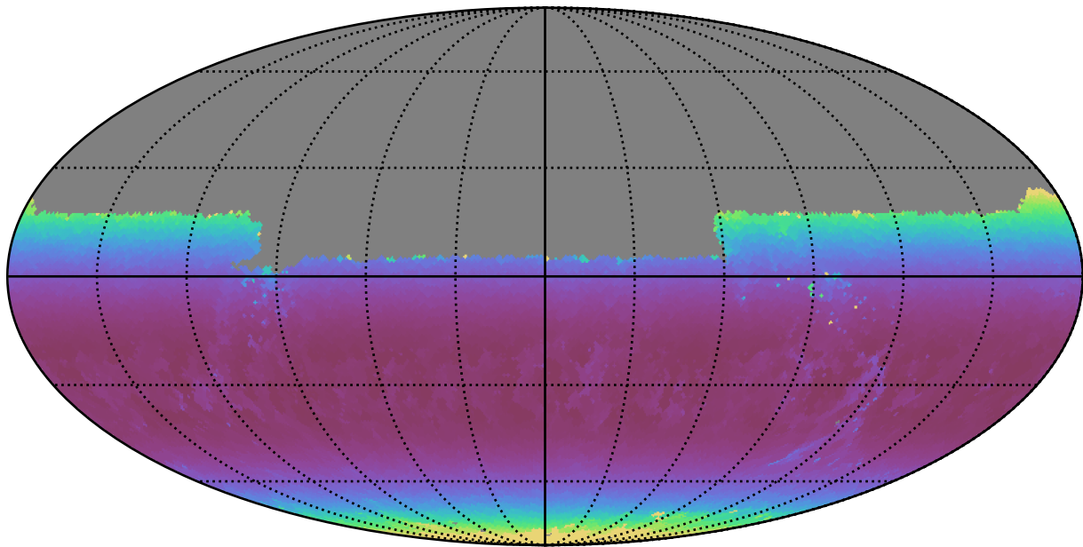
mw_roll_bulge_v3.3_10yrs Yr 1 y band: Min airmass
