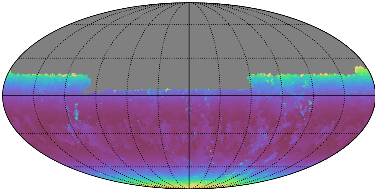
mw_roll_bulge_v3.3_10yrs Yr 1 u band: Min airmass
