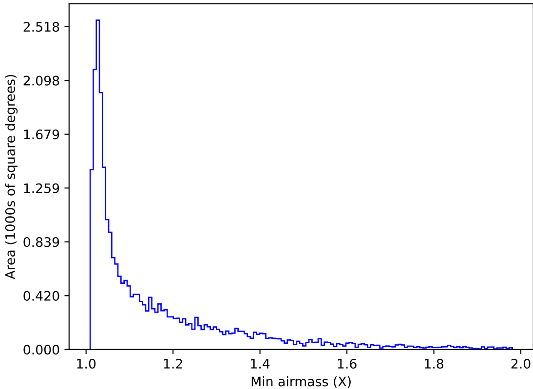
mw_roll_bulge_v3.3_10yrs Yr 1 r band: Min airmass
