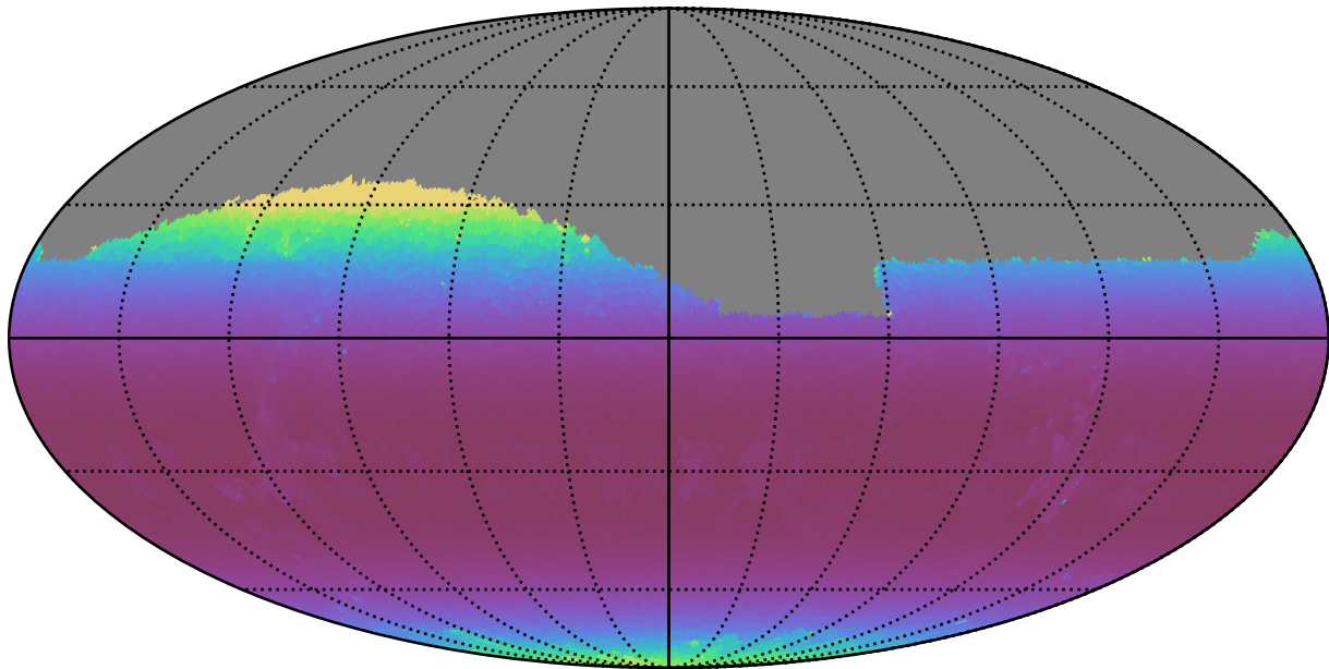
mw_roll_bulge_v3.3_10yrs Yr 1 i band: Min airmass
