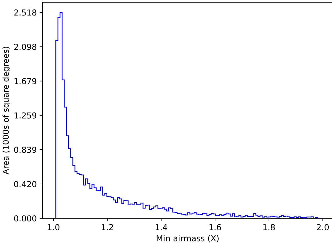
mw_roll_bulge_v3.3_10yrs Yr 1 i band: Min airmass
