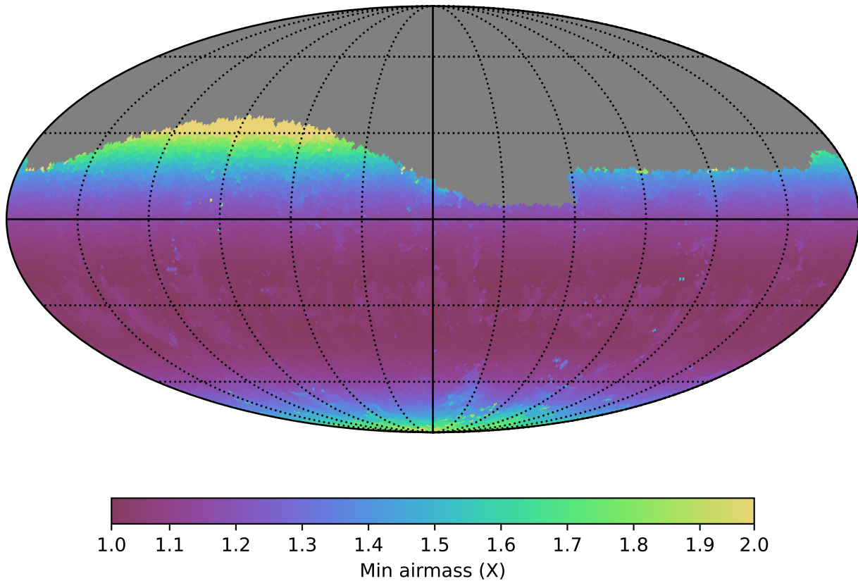
mw_roll_bulge_v3.3_10yrs Yr 1 g band: Min airmass
