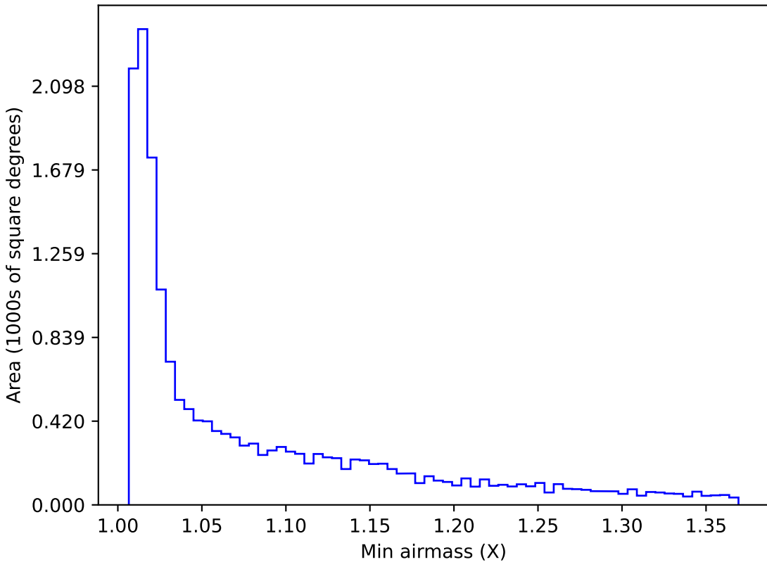
mw_roll_bulge_v3.3_10yrs WFD z band: Min airmass
