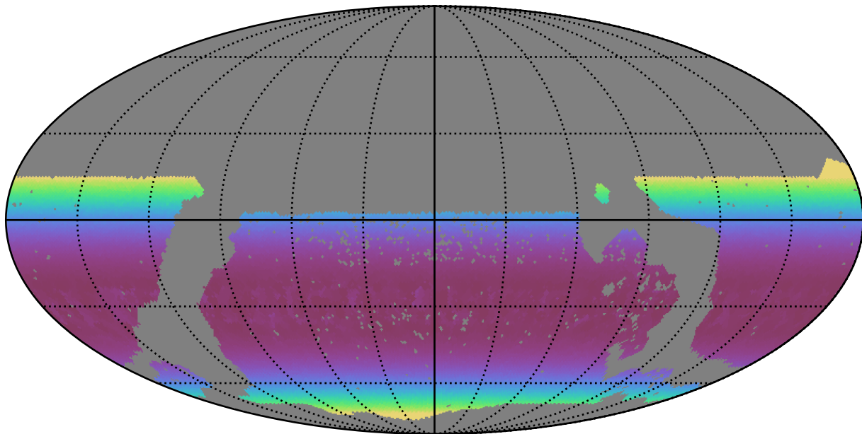
mw_roll_bulge_v3.3_10yrs WFD y band: Min airmass
