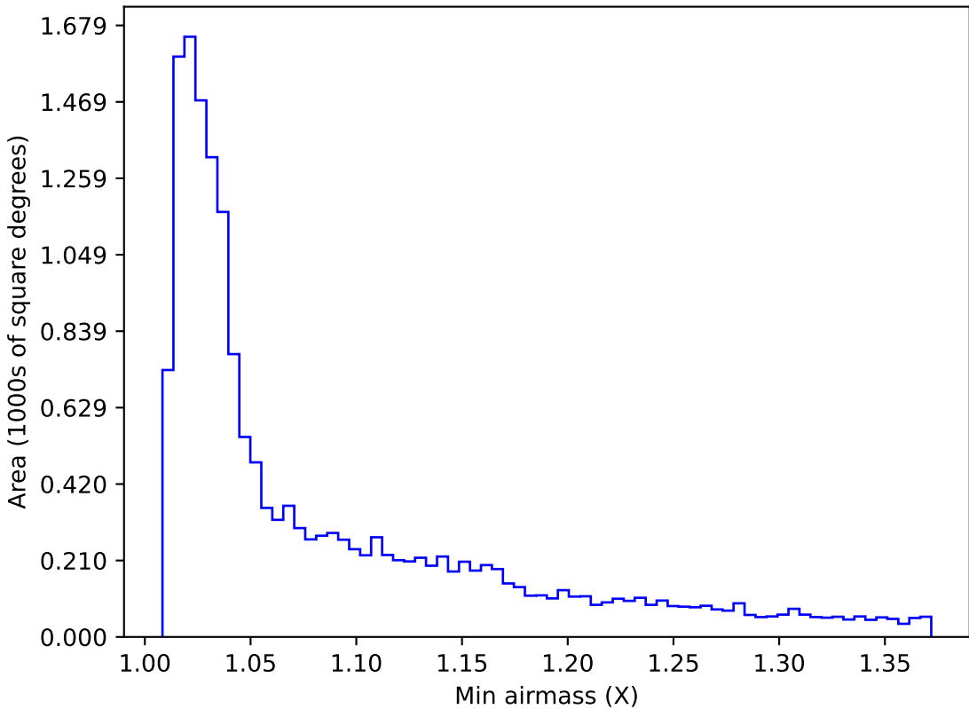
mw_roll_bulge_v3.3_10yrs WFD u band: Min airmass
