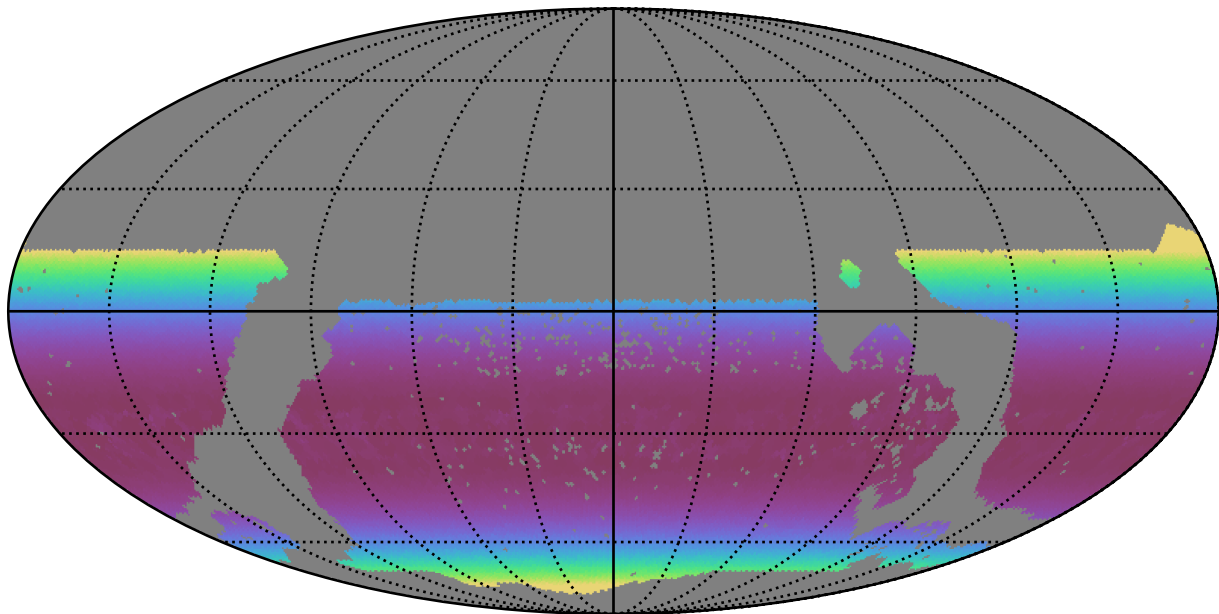
mw_roll_bulge_v3.3_10yrs WFD r band: Min airmass
