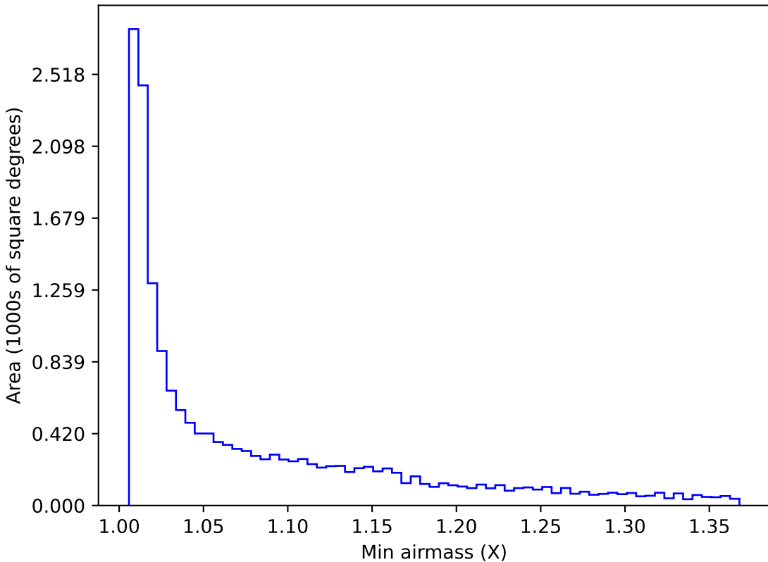
mw_roll_bulge_v3.3_10yrs WFD i band: Min airmass
