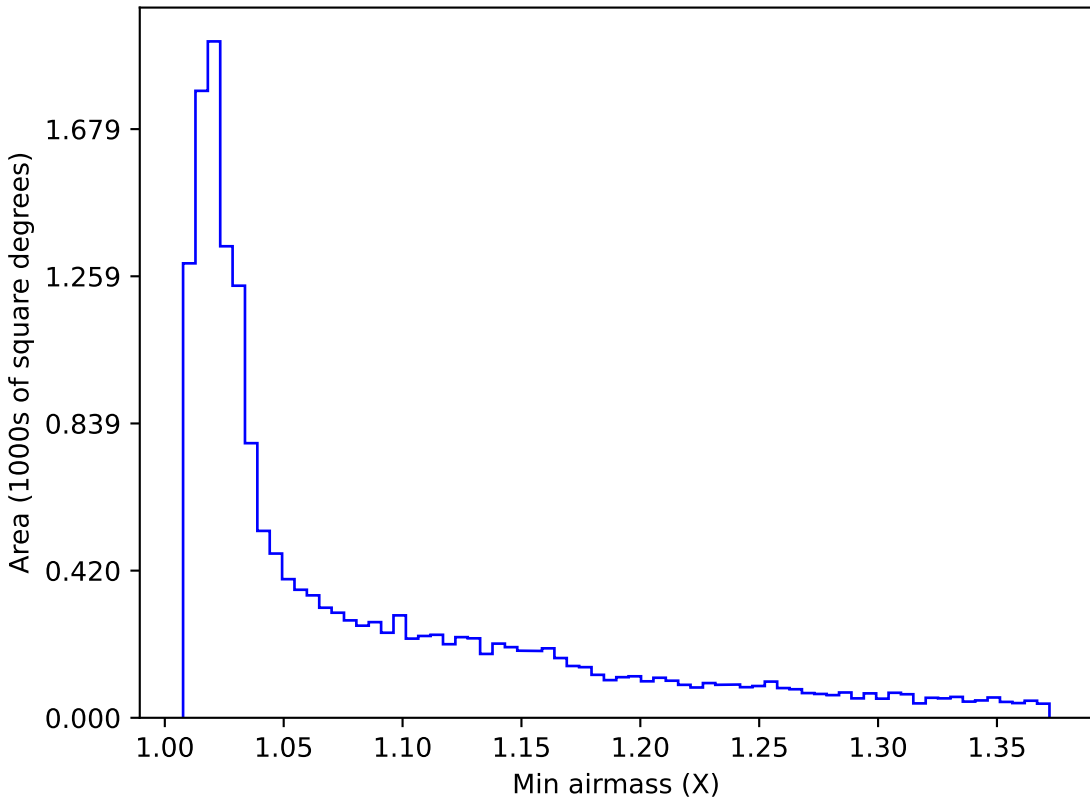
mw_roll_bulge_v3.3_10yrs WFD g band: Min airmass
