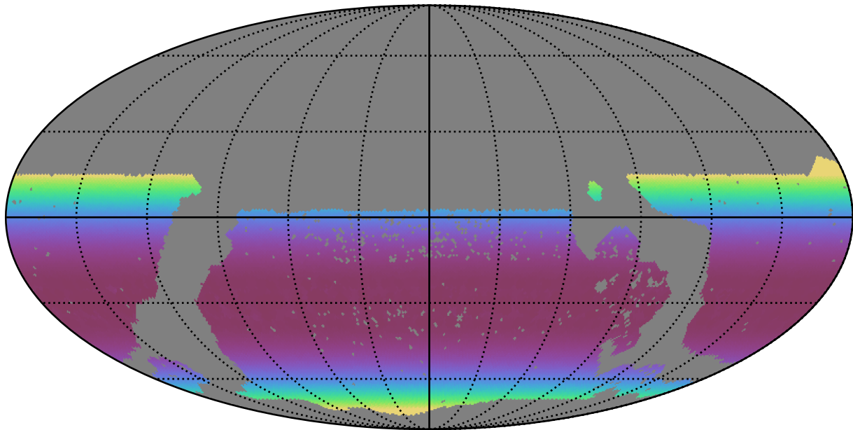
mw_roll_bulge_v3.3_10yrs WFD all bands: Min airmass
