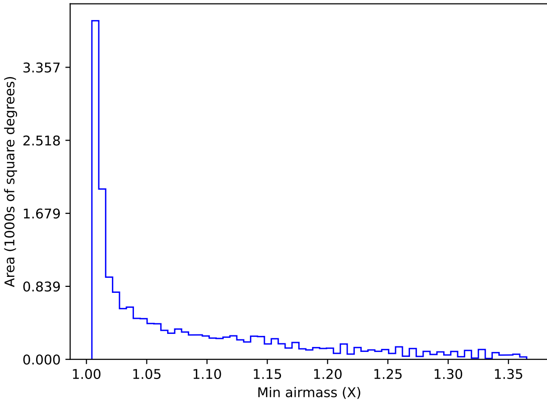
mw_roll_bulge_v3.3_10yrs WFD all bands: Min airmass
