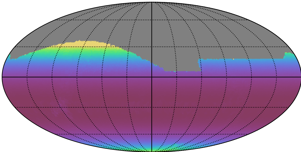
mw_roll_bulge_v3.3_10yrs All sky z band: Min airmass
