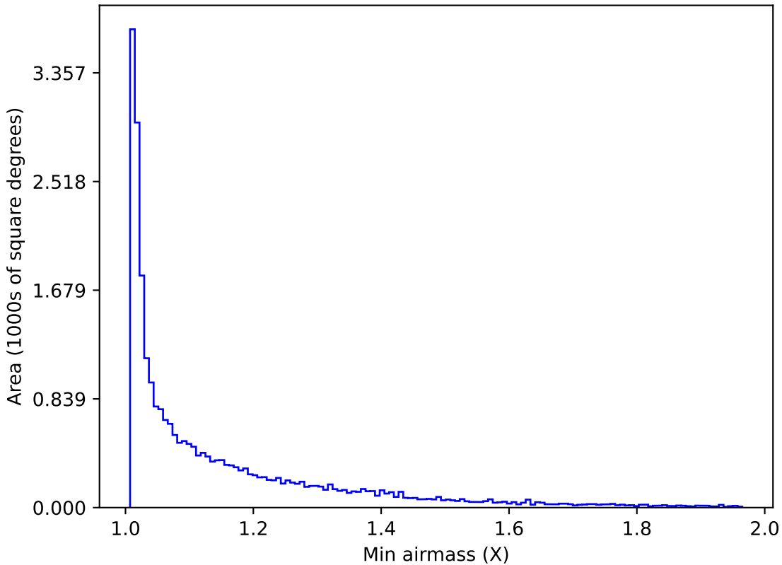
mw_roll_bulge_v3.3_10yrs All sky z band: Min airmass
