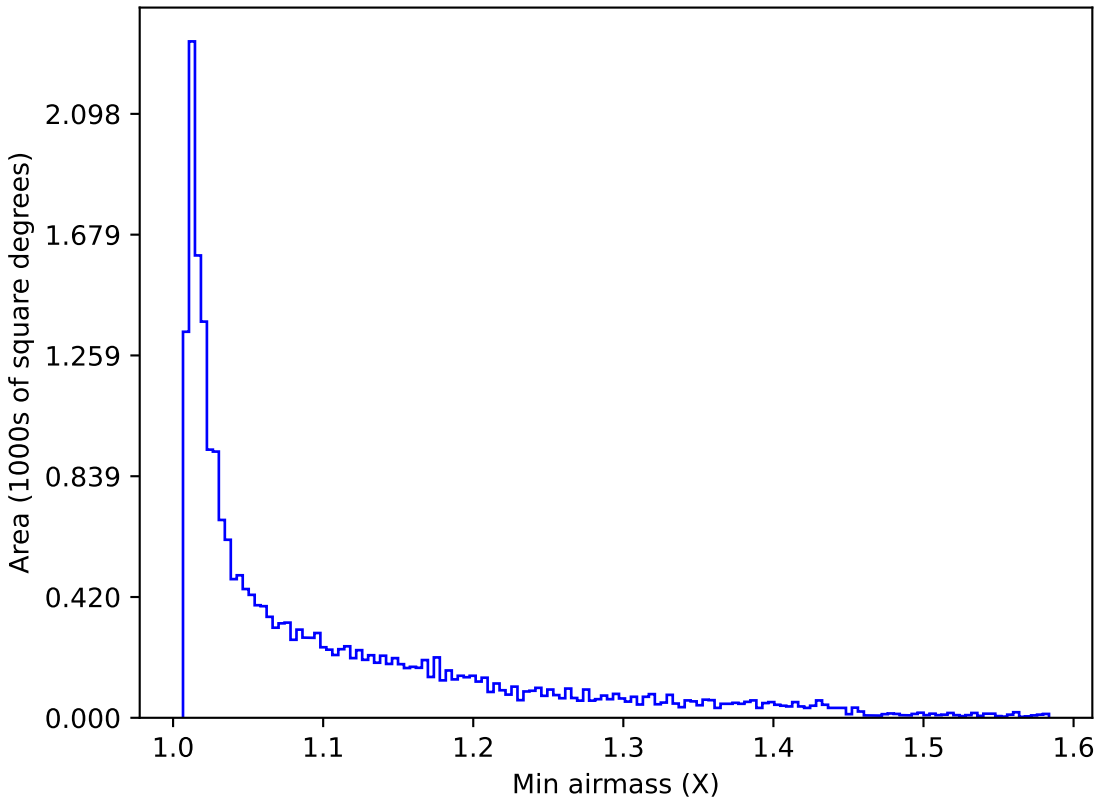
mw_roll_bulge_v3.3_10yrs All sky y band: Min airmass
