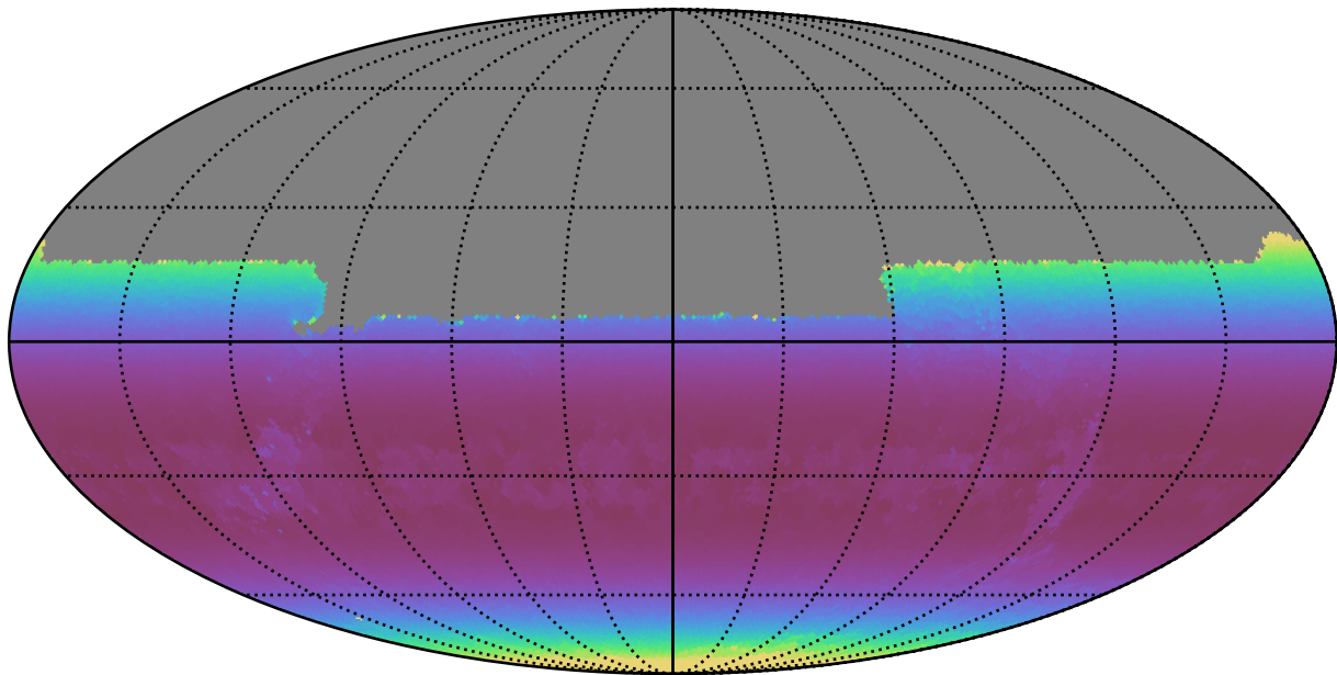
mw_roll_bulge_v3.3_10yrs All sky u band: Min airmass
