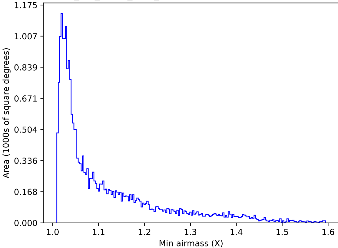
mw_roll_bulge_v3.3_10yrs All sky u band: Min airmass
