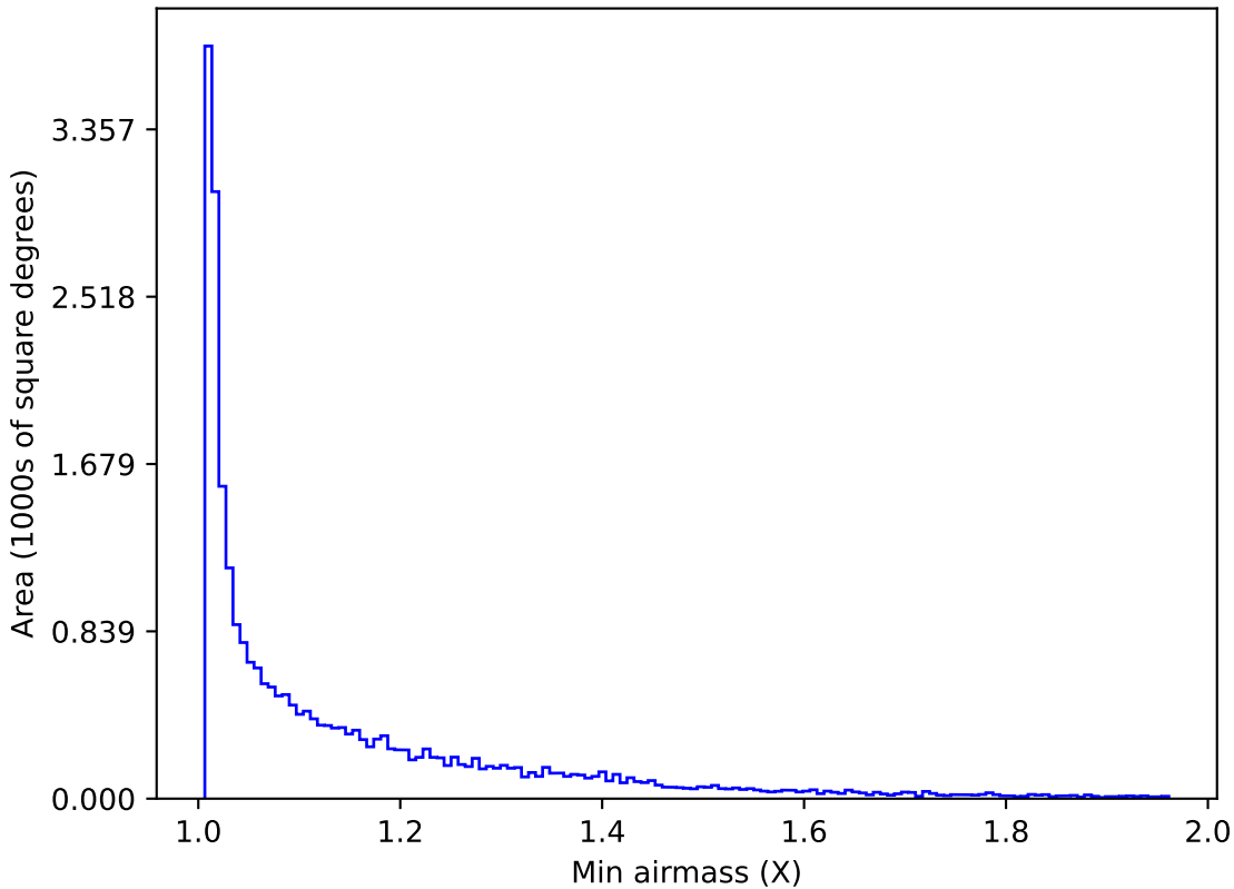
mw_roll_bulge_v3.3_10yrs All sky r band: Min airmass
