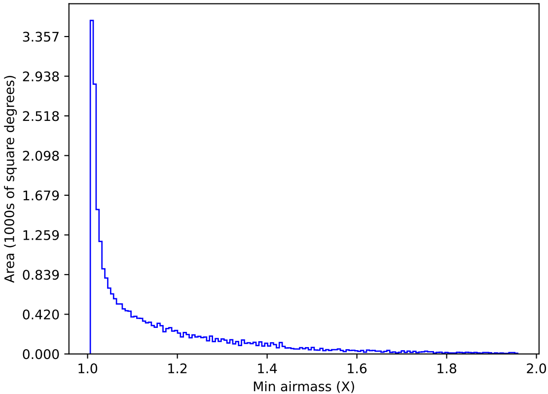
mw_roll_bulge_v3.3_10yrs All sky i band: Min airmass
