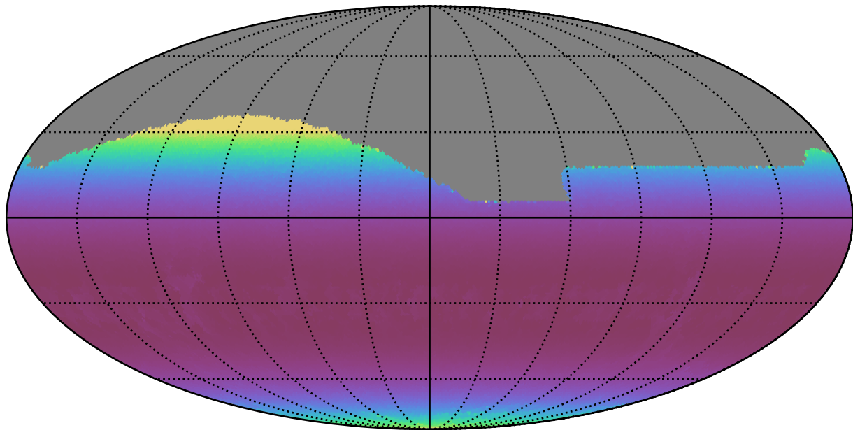
mw_roll_bulge_v3.3_10yrs All sky g band: Min airmass
