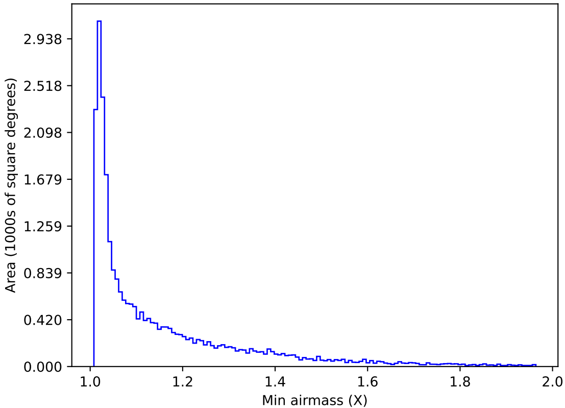
mw_roll_bulge_v3.3_10yrs All sky g band: Min airmass
