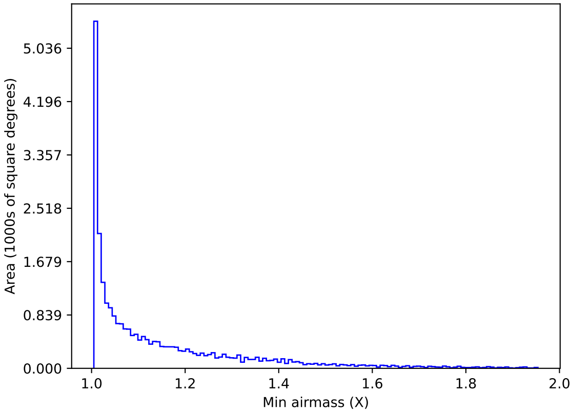
mw_roll_bulge_v3.3_10yrs All sky all bands: Min airmass
