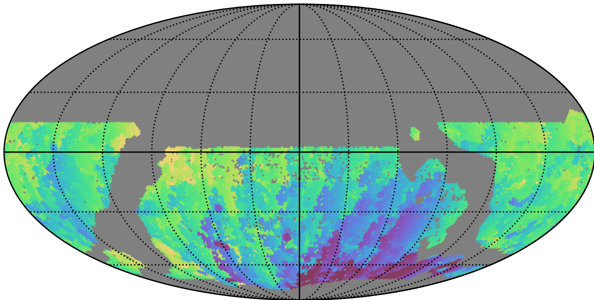
mw_roll_bulge_v3.3_10yrs WFD u band: Min HA
