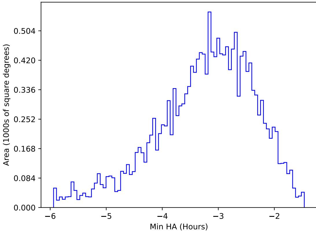
mw_roll_bulge_v3.3_10yrs WFD u band: Min HA
