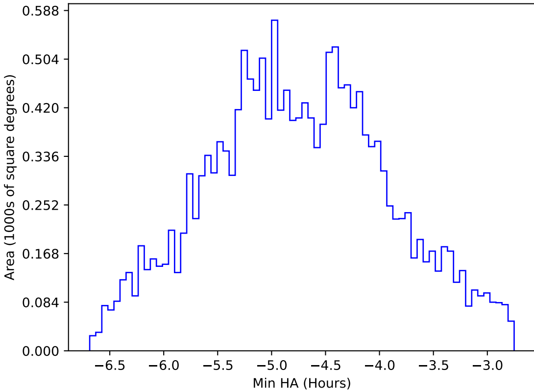
mw_roll_bulge_v3.3_10yrs WFD all bands: Min HA
