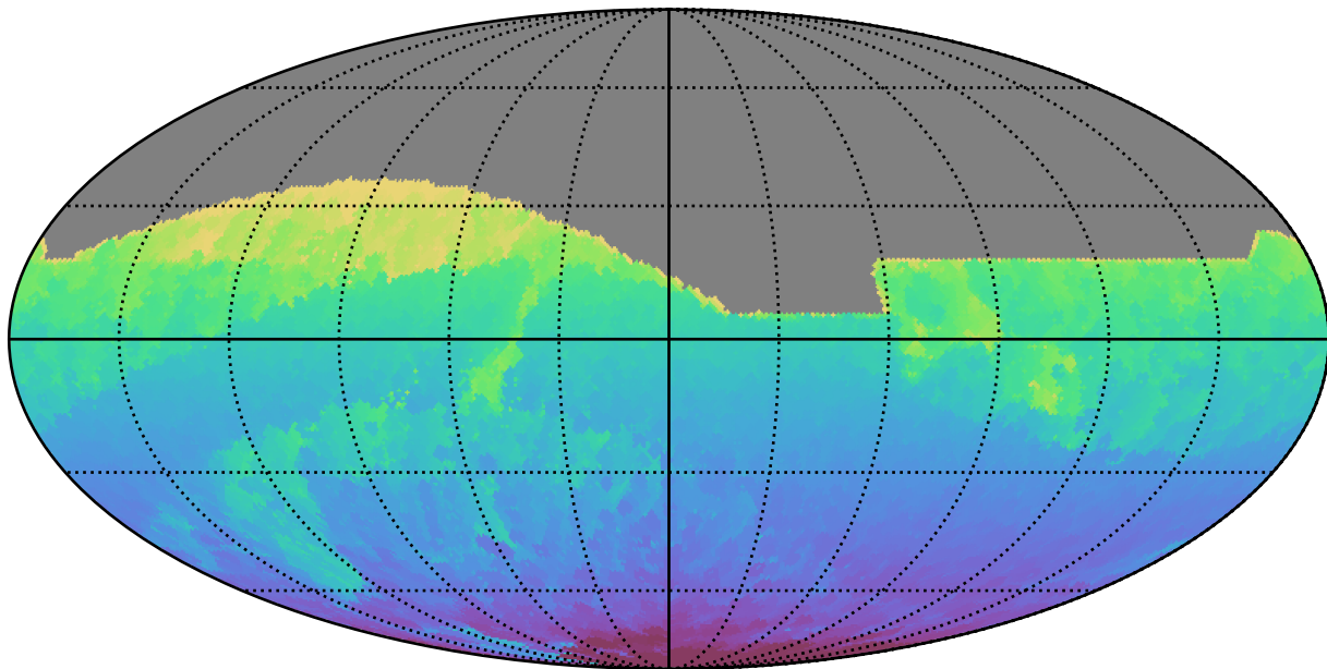
mw_roll_bulge_v3.3_10yrs All sky all bands: Min HA
