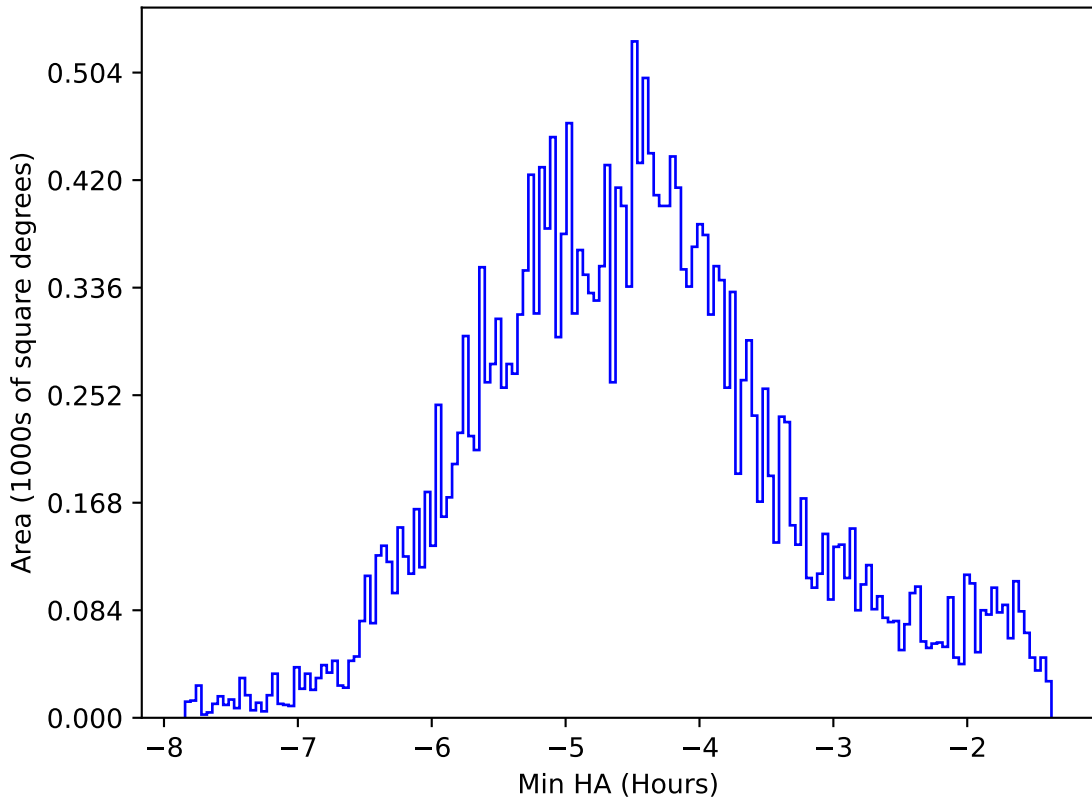
mw_roll_bulge_v3.3_10yrs All sky all bands: Min HA
