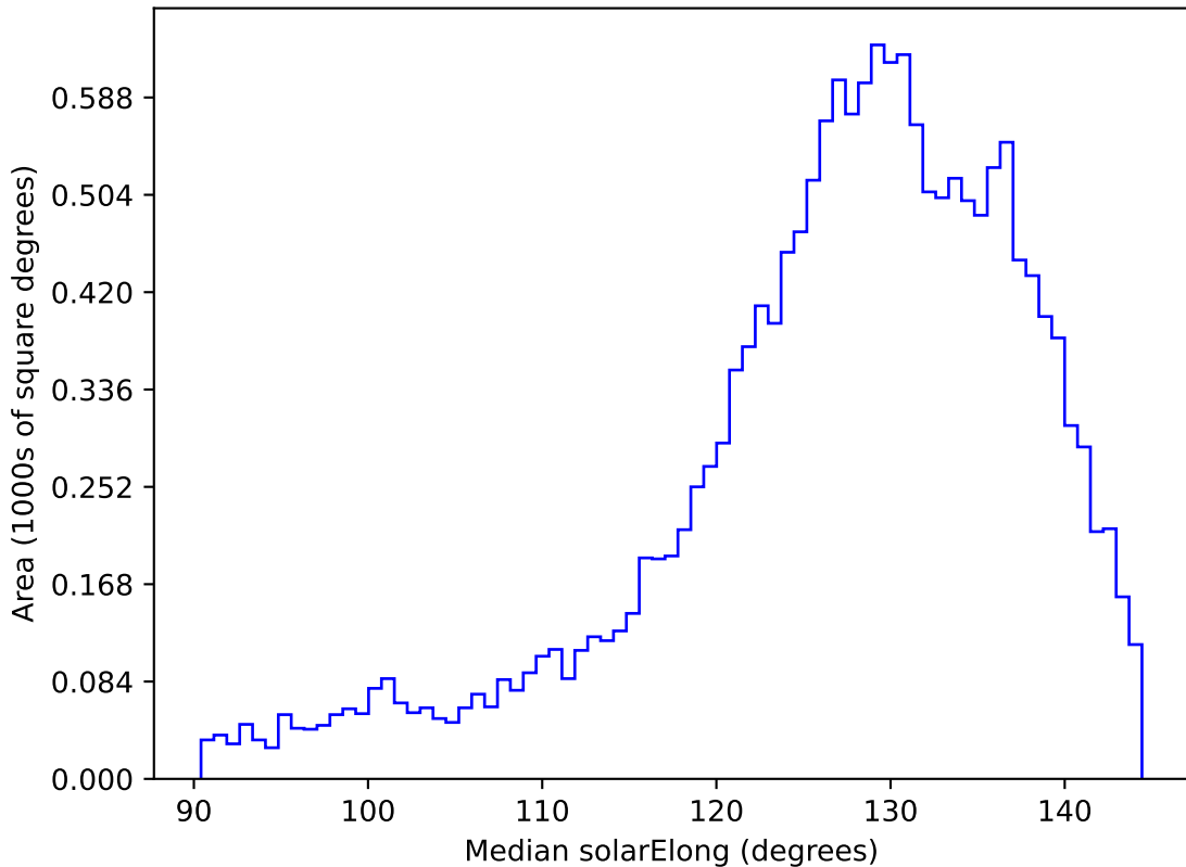
mw_roll_bulge_v3.3_10yrs WFD z band: Median solarElong
