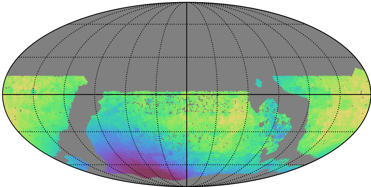
mw_roll_bulge_v3.3_10yrs WFD y band: Median solarElong
