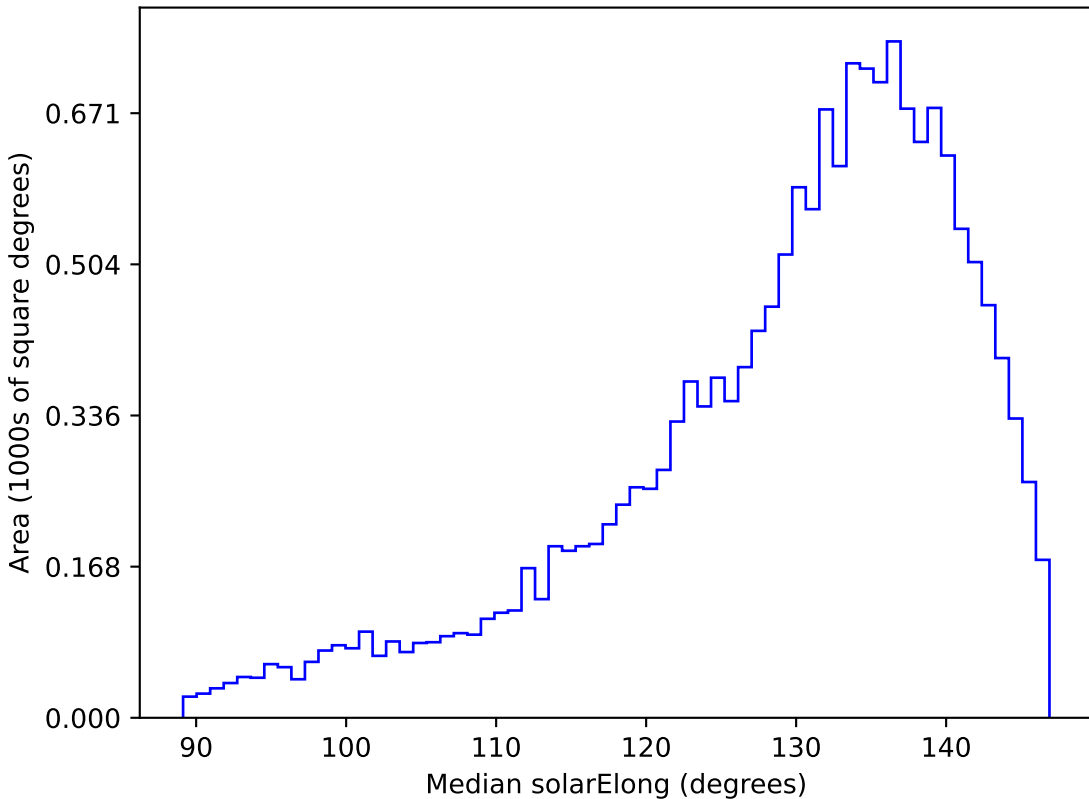
mw_roll_bulge_v3.3_10yrs WFD y band: Median solarElong
