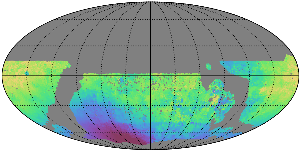
mw_roll_bulge_v3.3_10yrs WFD u band: Median solarElong
