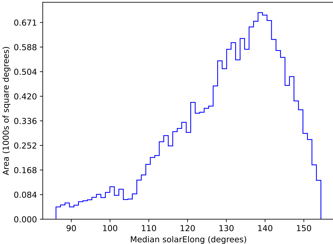
mw_roll_bulge_v3.3_10yrs WFD u band: Median solarElong
