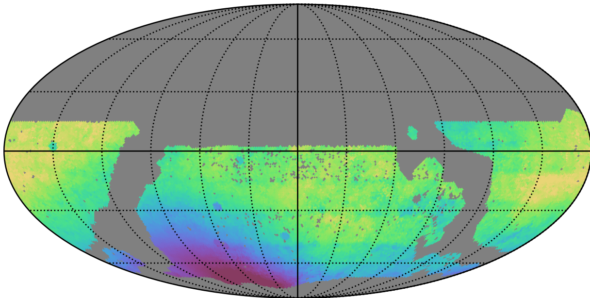
mw_roll_bulge_v3.3_10yrs WFD r band: Median solarElong
