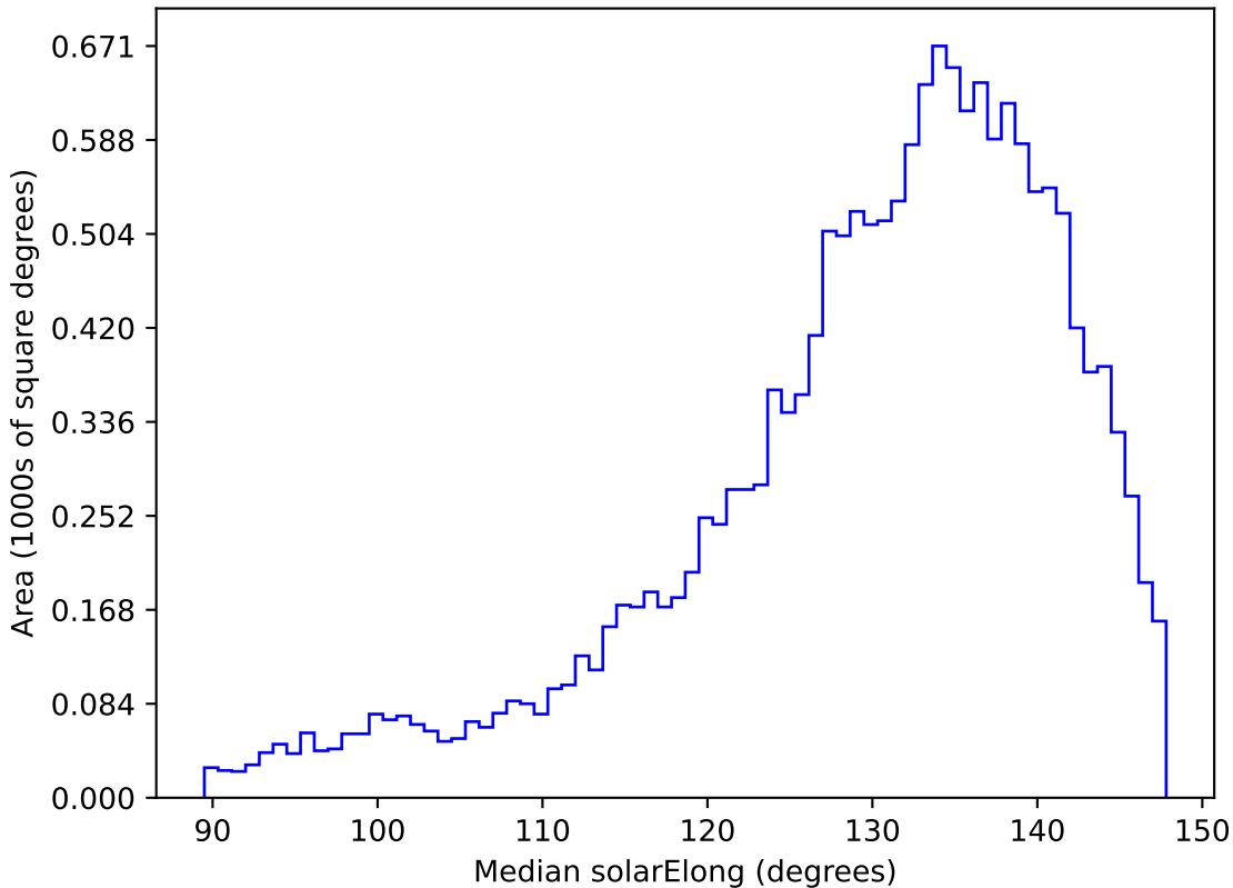
mw_roll_bulge_v3.3_10yrs WFD r band: Median solarElong
