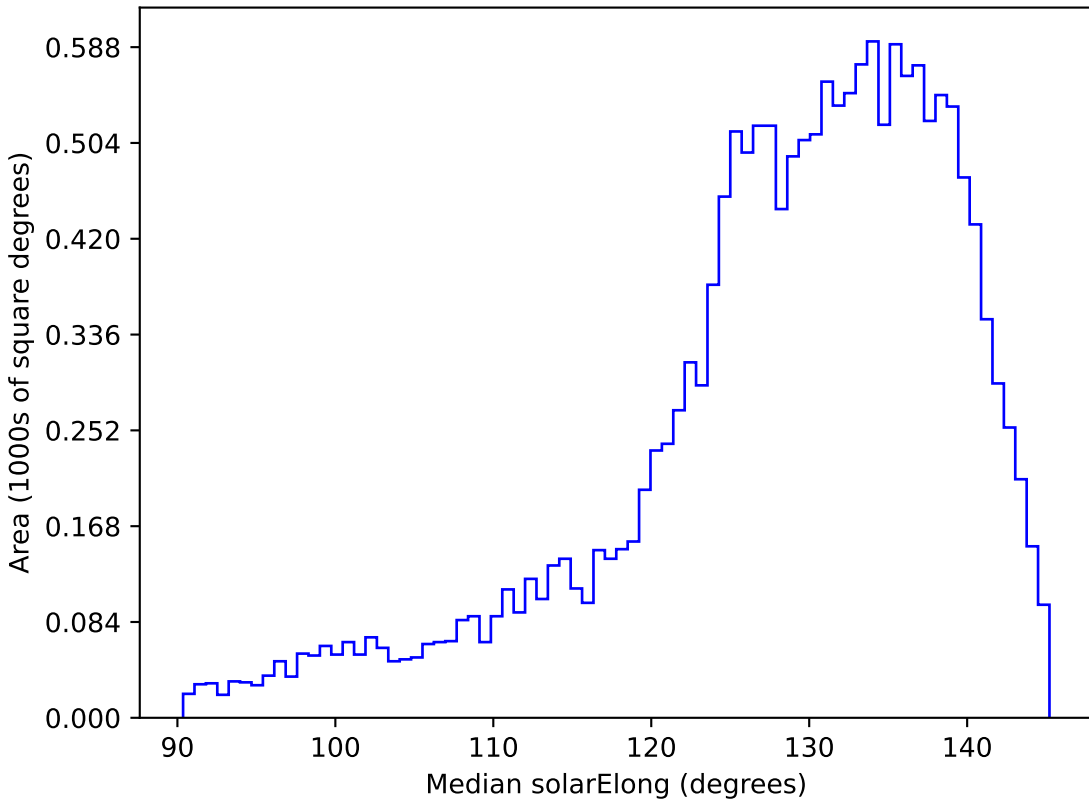
mw_roll_bulge_v3.3_10yrs WFD i band: Median solarElong
