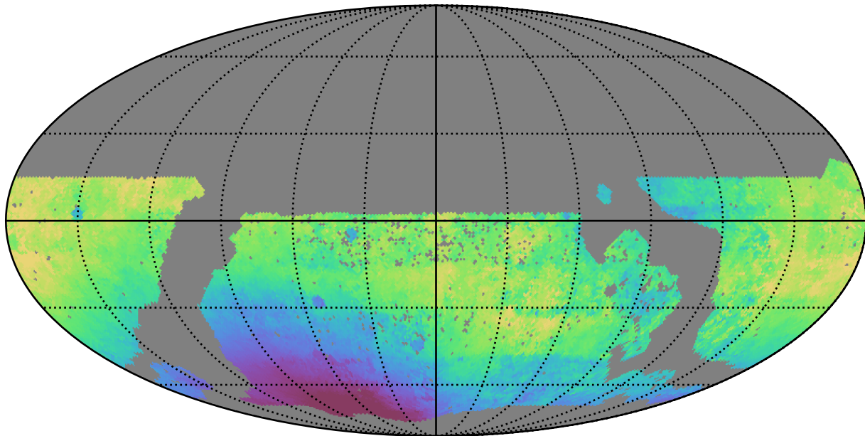
mw_roll_bulge_v3.3_10yrs WFD g band: Median solarElong
