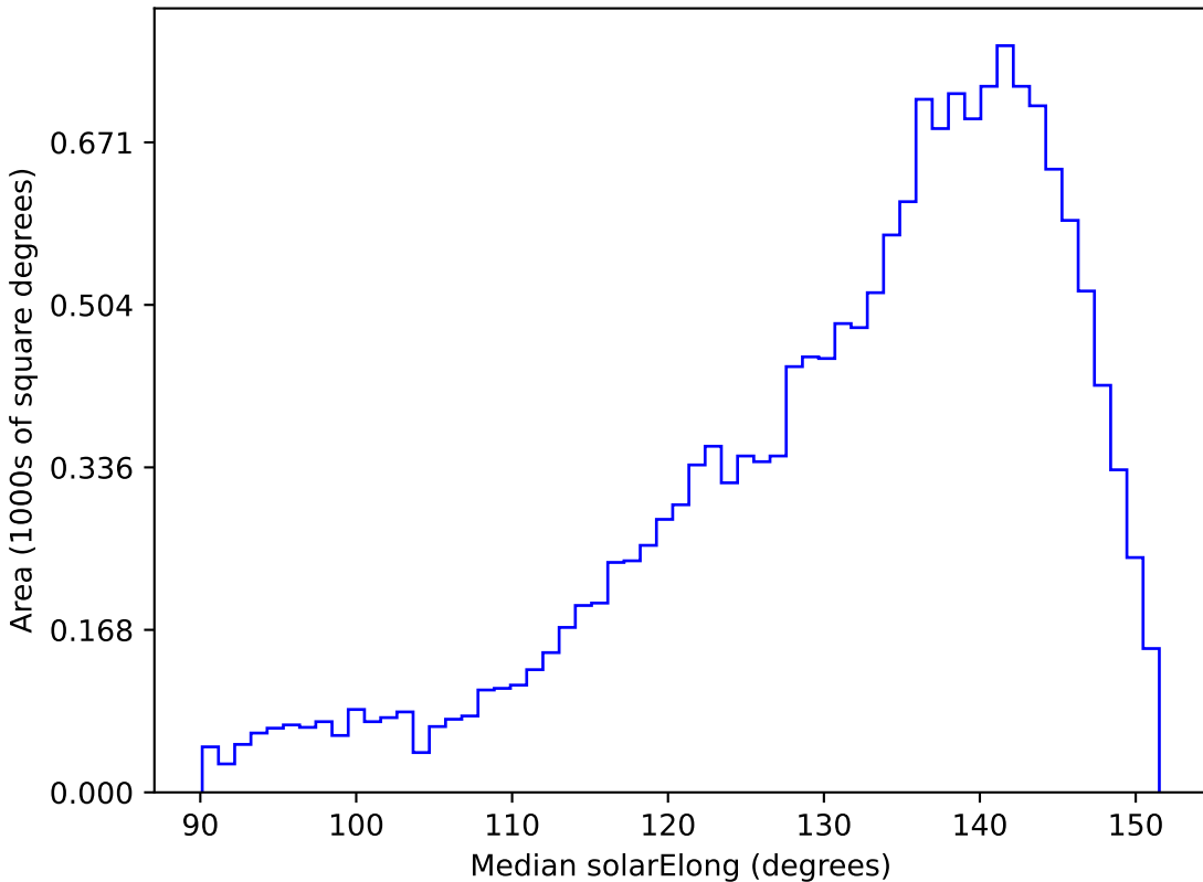
mw_roll_bulge_v3.3_10yrs WFD g band: Median solarElong
