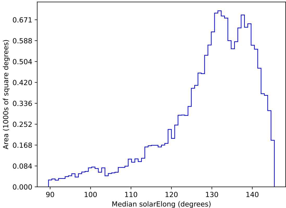
mw_roll_bulge_v3.3_10yrs WFD all bands: Median solarElong
