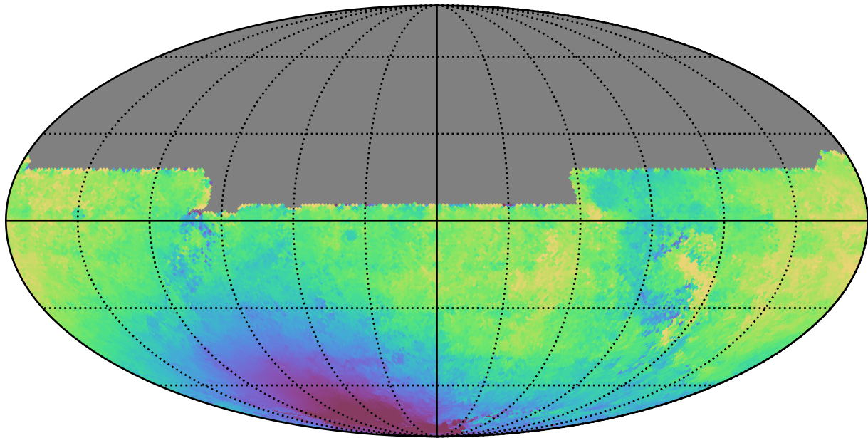
mw_roll_bulge_v3.3_10yrs All sky y band: Median solarElong
